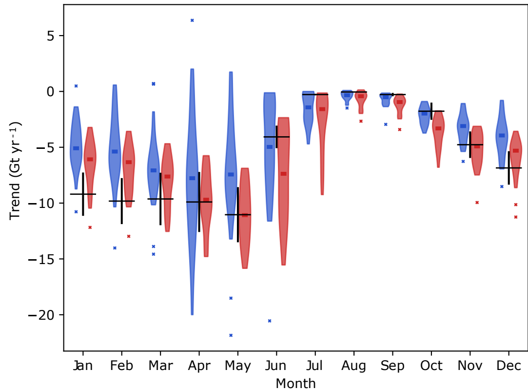
(b) 1981–2014 NH snow mass trend
