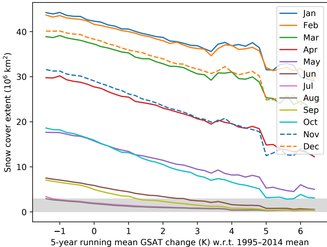
CMIP6 NH snow cover extent (historical+ssp585)
