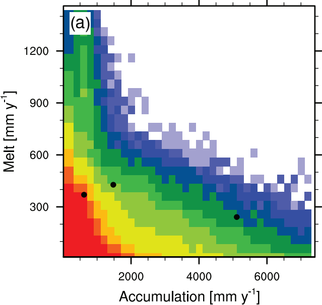
IMAU-FDM climatology
