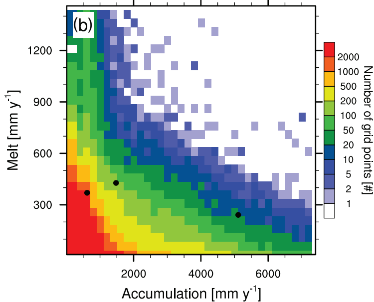
SNOWPACK climatology
