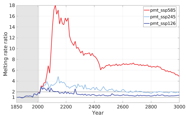
Figure 4. Melting rate ratios relative to pmt_pre for the main scenarios. The 10-year averages. Grey shading marks the historical period.
