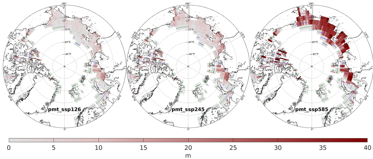
Figure 5. SSPF ice column melting for the three main experiments in the period 1850–3000. Green dots mark points entirely without SSPF ice, and blue dots mark points where all SSPF ice melted before the year 3000.
