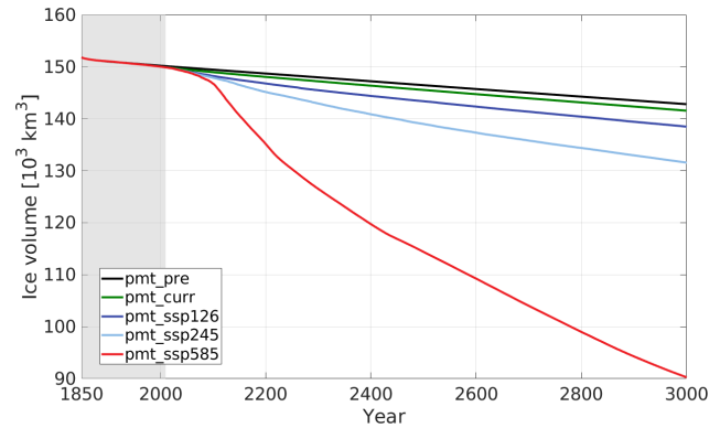
Figure 3. Volume of pan-Arctic SSPF ice for the scenario and control experiments. Grey shading marks the historical period.
