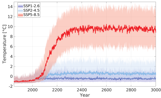
Figure 2. Benthic temperature. Lines are yearly averages over the area containing SSPF ice in 1850. Shaded areas show decadal means of the extreme months for each year and are combined RGB-wise.
