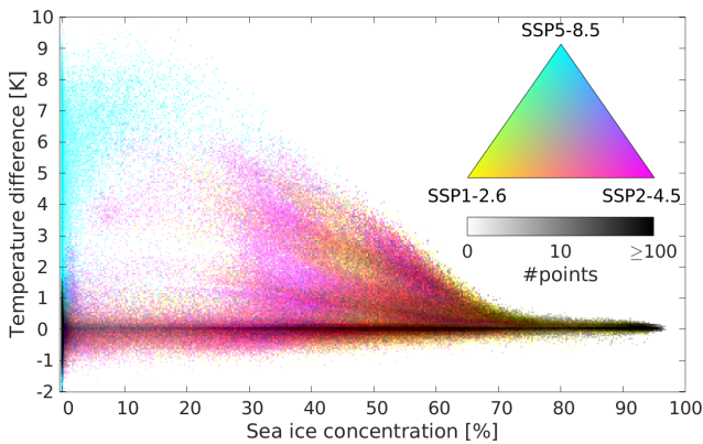
Figure 8. Temperature difference between ocean bottom (“benthic” temperature) and the uppermost subsea sediment layer as a function of fractional local sea ice concentration for the scenario experiments. Logarithmic density plot (temperature difference in 0.05 K bins, sea ice cover in 0.25 % bins) of monthly mean values. The colours are combined RGB-wise according to the colour triangle. The colour saturation is scaled such that 0 points in a bin correspond to the value 0, and \geq 100 points correspond to the value 1. Thus for instance a red point contains an equal number of points from pmt_ssp126 and pmt_ssp245 but none from pmt_ssp585 . Black indicates at least 100 points in all three scenarios. Each scenario contributes more than 460 000 time–space points.
