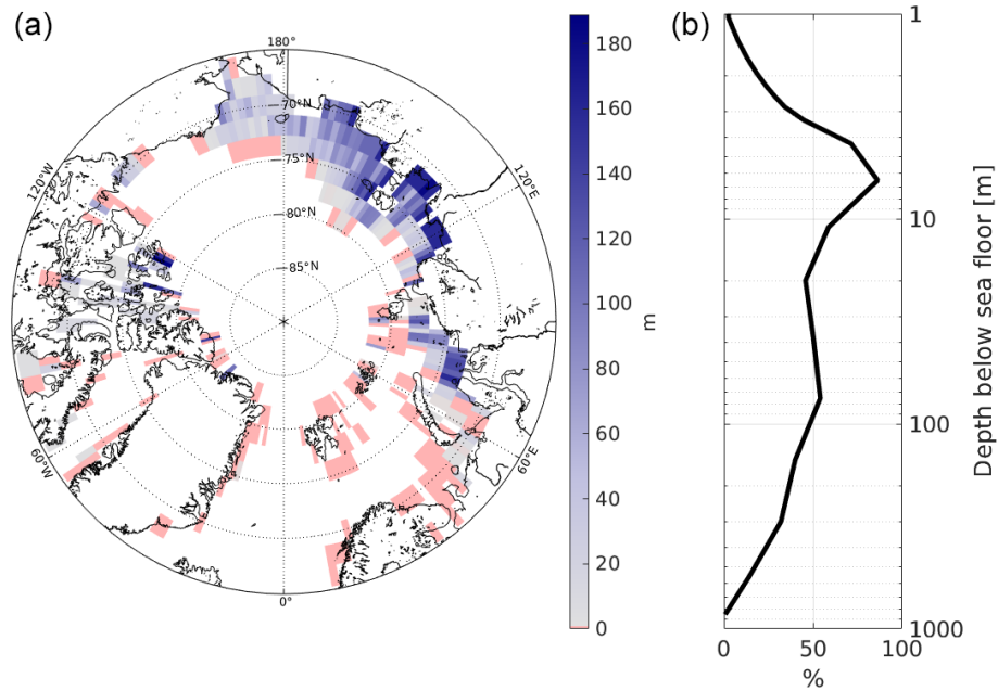
Figure 1. (a) Length of initial (1850) SSPF ice column. Reddish colour marks points entirely without ice in the sediments. (b) Vertical distribution of initial ice concentration in sediment pore space (SSPF ice saturation). Panel (b) shows the spatial average over the area containing SSPF ice in 1850.
