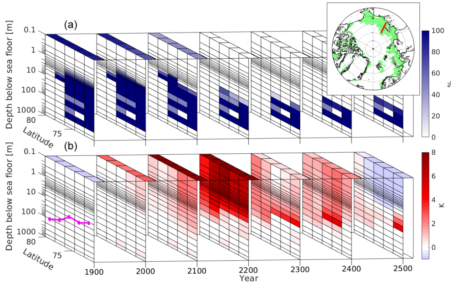
Figure 7. SSPF ice saturation (a, lat–depth planes), sea ice concentration (a, lat–time planes), sediment temperature change (b, lat–depth planes), and atmospheric 2 m temperature change (b, lat–time planes) along a section across the East Siberian Shelf (153° E, shown on the insert in a) for different time periods. In (b) time slice at 1900 represents the 1850–1900 change, and subsequent slices represent the changes relative to the slice before. Black lines at constant depth are model layer boundaries. Magenta line shows the water depth along the section. Shown are (differences between) yearly averages.
