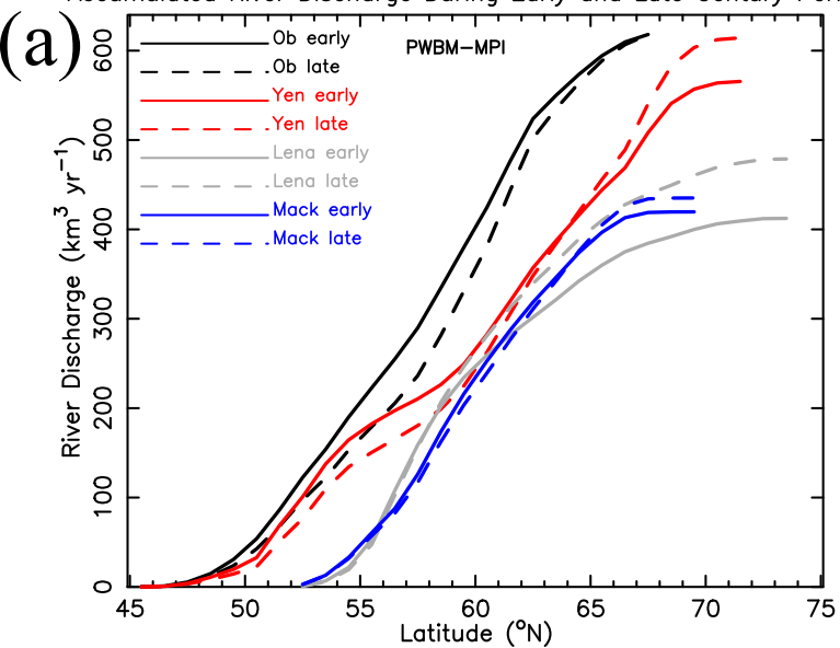
Accumulated River Discharge During Early and Late Century Periods
