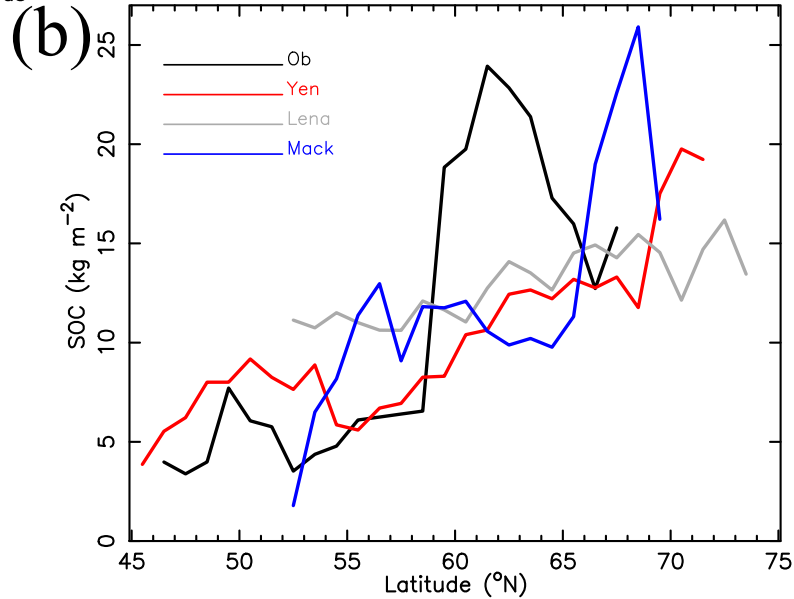
Soil Organic Carbon Storage, 0–200 cm
