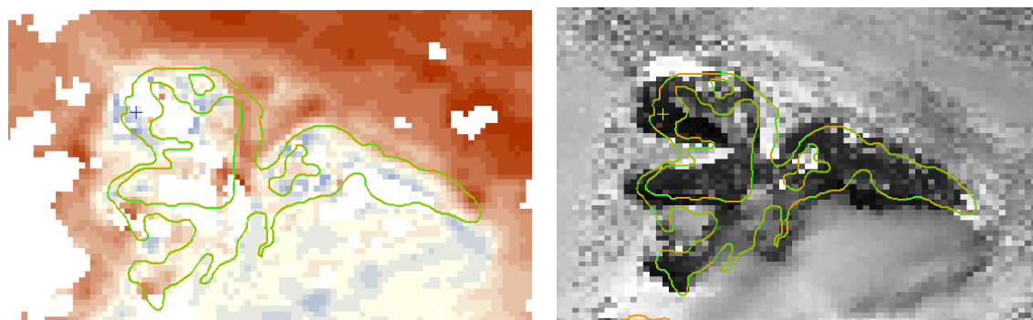
Figure S5. A large nunatak area in the dDEM image (left) and a single SPOT-5 image (right). Nunatak extent outline from the ADD is shown in green. The dimensions of the box are about 1 km by 0.5 km.
