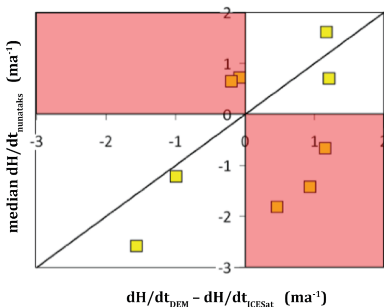
Figure S3: Analysis of dH/dt from the two methods for data near nunatak areas in high-mass-loss basins within the study area.
