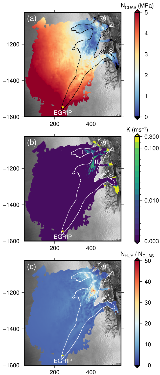
Figure 9. Results for NEGIS region with forcing due to basal melt (PISM) \tau -representing winter conditions. White lines indicate the 50 \text{m a}^{-1} velocity contour. Panel (a) shows effective pressure N_{CUAS} , (b) conductivity K (logarithmic scale), and (c) shows the quotient of the ice overburden pressure above flotation and the effective pressure computed by CUAS.
