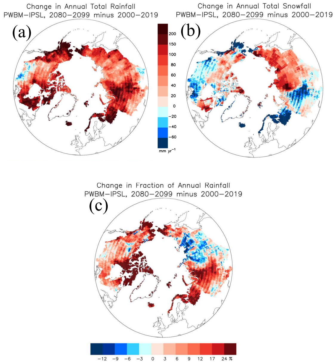
Figure S4: Change in (a) annual rainfall ( \text{mm yr}^{-1} ), (b) snowfall ( \text{mm yr}^{-1} ), and (c) the fraction of rainfall to total precipitation from PWBM-IPSL simulation.
