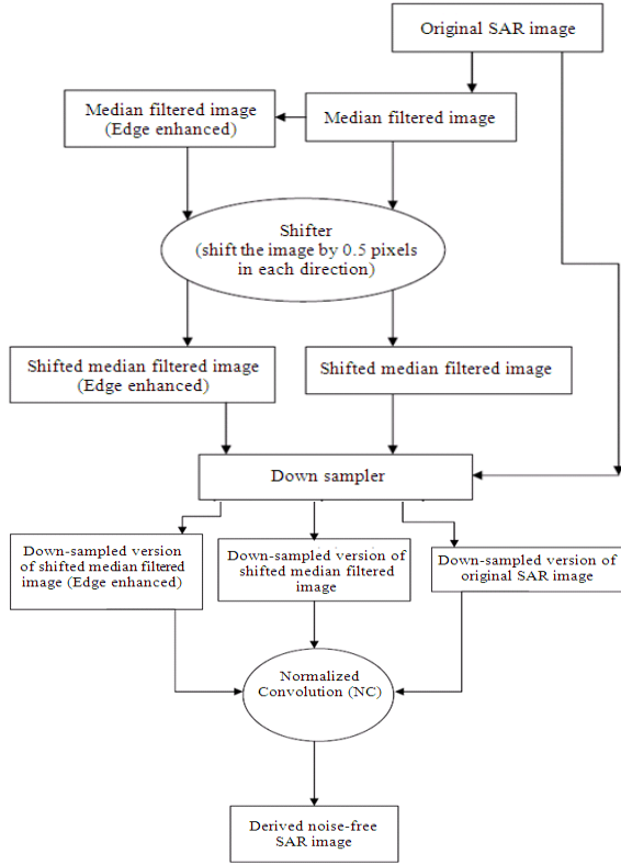
Fig. 1: Flow chart for proposed SAR image de-noise system
