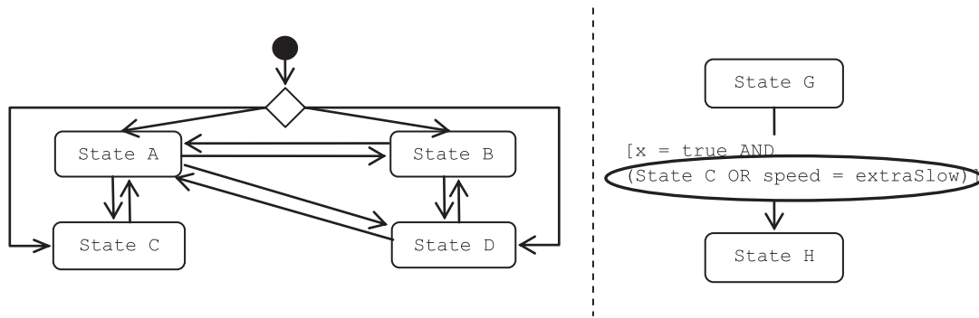
Fig. 7. Incorrect guard on transition from State G to State H.
