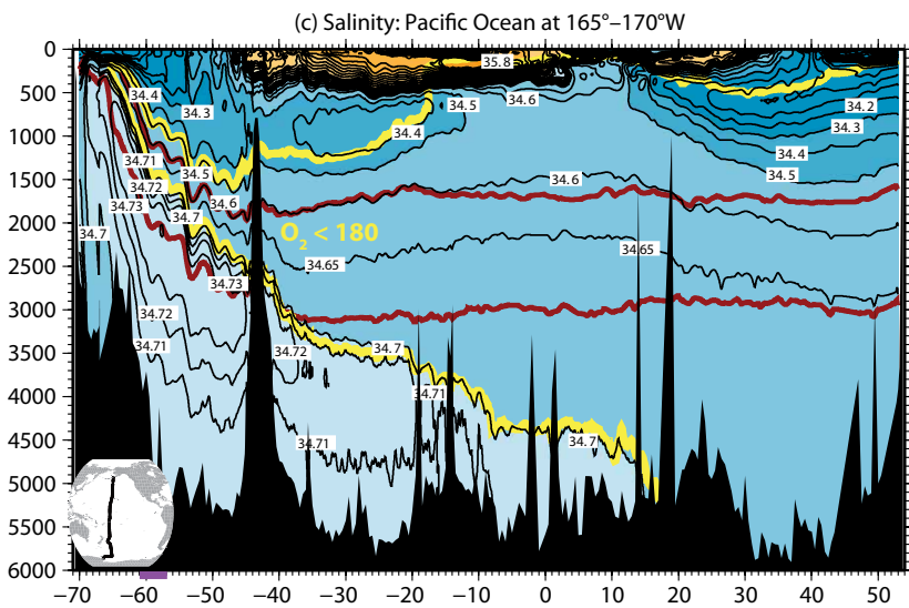
Figure 2. Salinity for the (a) Atlantic (20°–25°W), (b) Indian (80°–95°E), and (c) Pacific (165°–170°W) Oceans. The 180 \text{ } \mu\text{mol kg}^{-1} oxygen contour (heavy yellow) illustrates the oxygen minimum in the Southern Ocean, which originates in the Indian and Pacific Oceans (Indian Deep Water and Pacific Deep Water) and lies above the salinity maximum that originates in the North Atlantic (North Atlantic Deep Water). Isonneutral contours \gamma^N = 27.8 and 28.04 \text{ kg m}^{-3} (heavy dark red) represent the cores of the low oxygen Indian Deep Water/Pacific Deep Water and high-salinity North Atlantic Deep Water components, respectively. Section locations are indicated on inset maps. The heavy purple line segment on the latitude axes marks the Drake Passage latitude band (61°–57°S). For further information on these sections, including other measured properties and data sets, see the World Ocean Circulation Experiment atlases (Orsi and Whitworth, 2004; Talley, 2007, 2011; Koltermann et al., 2011).
