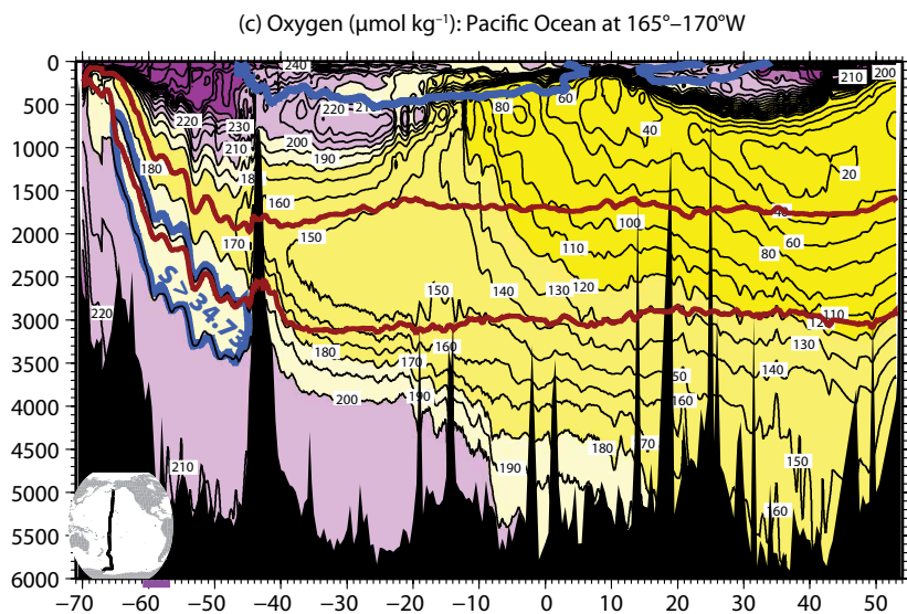
Figure 3. Oxygen ( \mu\text{mol kg}^{-1} ) for the (a) Atlantic (20°–25°W), (b) Indian (80°–95°E), and (c) Pacific (165°–170°W) Oceans. The 34.73 salinity contour (heavy blue) illustrates the salinity maximum in the Southern Ocean, which originates in the North Atlantic (North Atlantic Deep Water) and lies beneath the oxygen minimum that originates in the Indian and Pacific Oceans (Indian and Pacific Deep Waters). The accompanying salinity sections are shown in Figure 2. Isonutral contours \gamma^N = 27.8 and 28.04 \text{ kg m}^{-3} (heavy dark red) represent the cores of the low oxygen Indian Deep Water/Pacific Deep Water and high-salinity North Atlantic Deep Water components, respectively. Section locations are indicated on inset maps. The heavy purple line segment on the latitude axes marks the Drake Passage latitude band (61°–57°S). For further information on these sections, including other measured properties and data sets, see the World Ocean Circulation Experiment atlases (Orsi and Whitworth, 2004; Talley, 2007, 2011; Koltermann et al., 2011).
