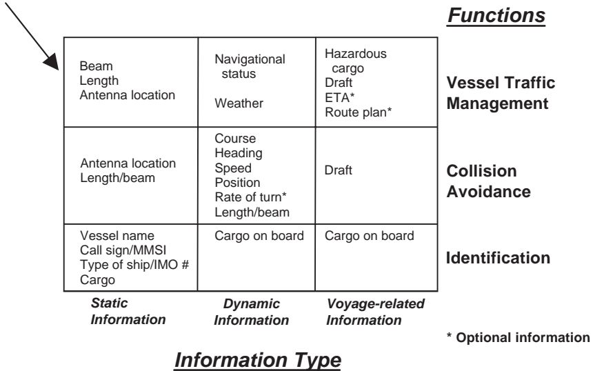
FIGURE 4-2 Representative AIS data elements, functions, and information.
