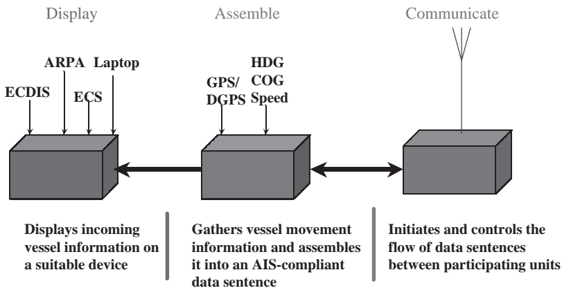
FIGURE 1-1 Elements of shipboard AIS. ARPA = automatic radar plotting aid; COG = course over ground; GPS = Global Positioning System; DGPS = Differential GPS; ECDIS = electronic charting and display information systems; ECS = electronic charting systems; HDG = heading. (Source: USCG 2001b.)
