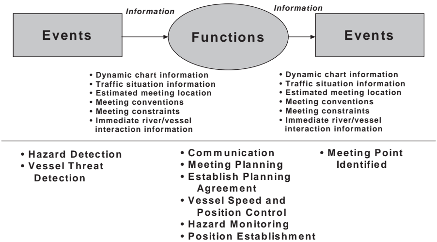
FIGURE 5-3 Towing vessel meeting example.
