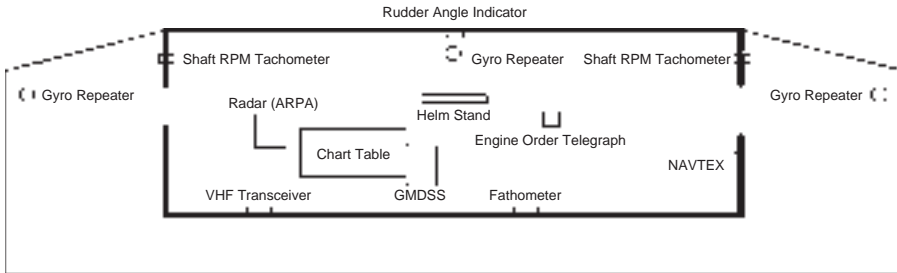
FIGURE 2-4 Typical wheelhouse layout of older ships. (GMDSS = Global Maritime Distress and Safety System.)
