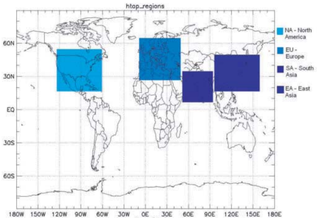
Figure 8.6 Source-receptor regions defined by the HTAP Task Force: (LRTAP, 2007).
