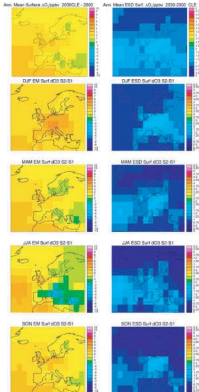
Figure 4.1 Left column: 26-model ensemble-mean change in annual mean surface ozone (top row) and 3-month seasonal mean surface ozone (subsequent rows) for year 2030 with “central” emissions scenario CLE (climate unchanged) (model run S2) compared with base year 2000 (model run S1). “DJF” refers to mean for the 3 months December, January, February, “MAM” refers to March April May, etc. Right column: Standard deviation of the corresponding 26-model ensemble simulations. Units are ppb ( 1 \text{ ppb } O_3 \equiv 2 \mu\text{g m}^{-3} O_3 ). The models have been interpolated to a common resolution ( 5^\circ \times 5^\circ horizontal); lowest model level depth is \sim 100 \text{ m} . Source: Stevenson (pers. comm., 2008) from data of Dentener et al. (2006).
