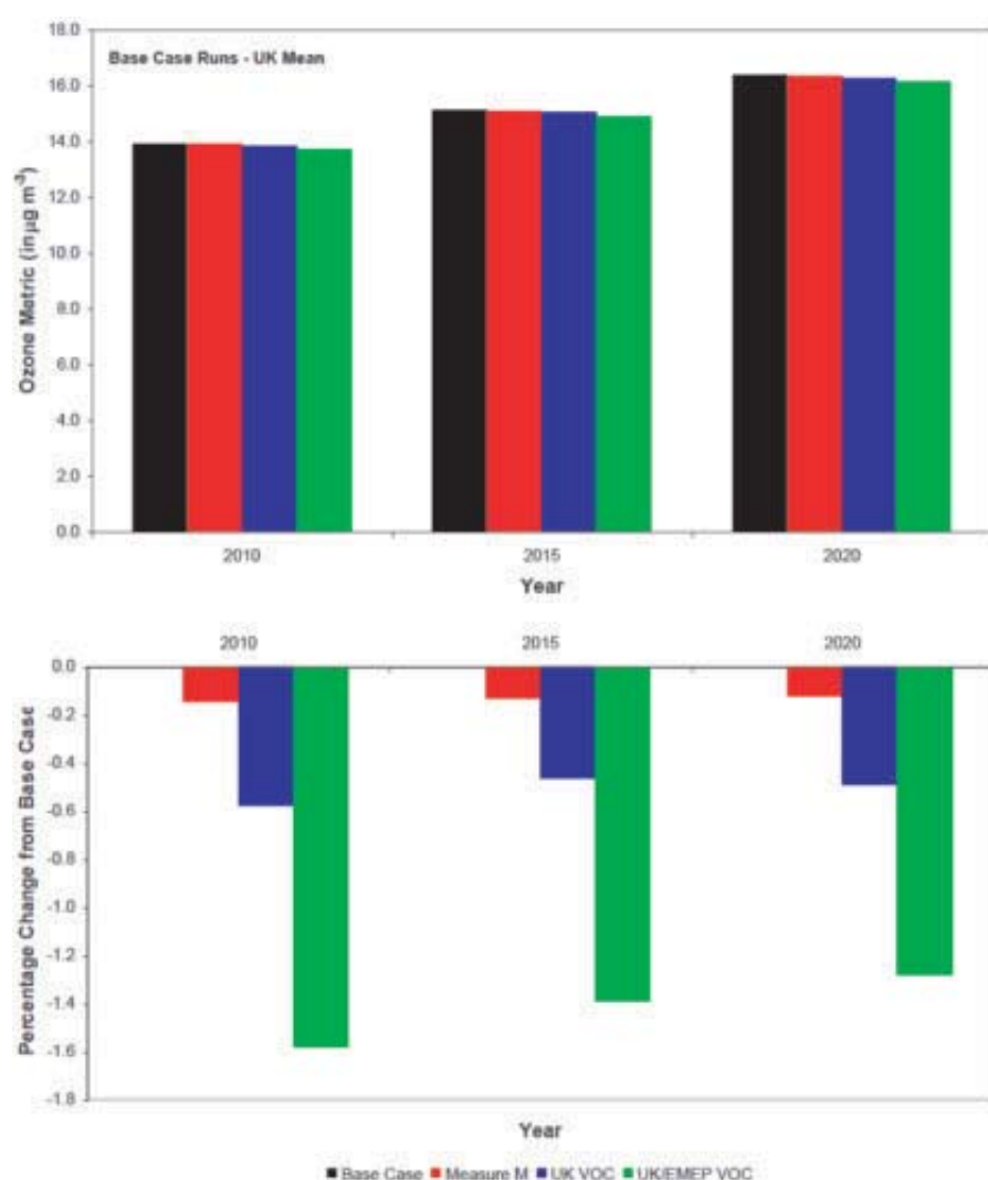
Figure 8.1 The response (upper panel) and percentage change from the base case (lower panels) of the metric – annual mean of the daily maximum of the 24 daily running 8-hour mean ozone concentrations using a 70 µg m -3 (i.e. 35 ppb) cut-off – calculated by the OSRM for the base case and for three VOC emission reduction scenarios: (a) Measure M in the Review of the UK Air Quality Strategy; (b) equivalent 9% across-the-board reductions of UK VOC emissions; and (c) 9% across-the-board reductions of UK and non-UK VOC emissions.
