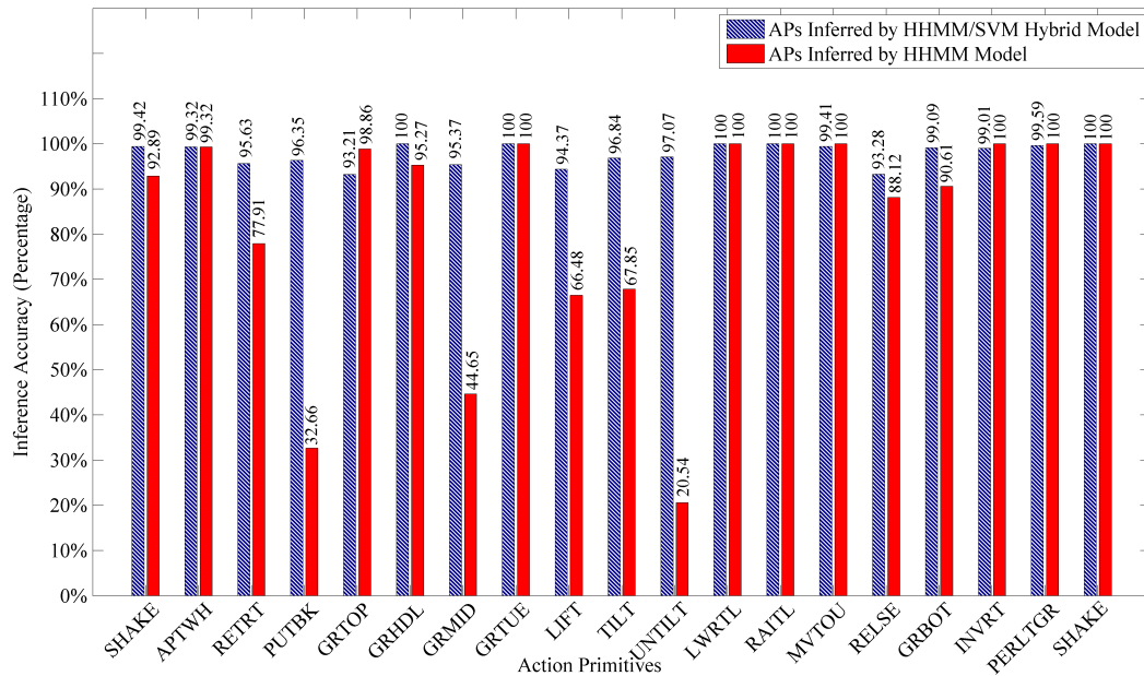
Fig. 7 APs inference accuracy by HHMM and HHMM/SVM Hybrid Models
