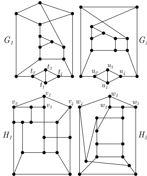
Figure 3. The top left graph G_1 is cospectral with the top right graph G_2 with the replaceable vertices (t_1, u_1, g) . The bottom left graph H_1 is cospectral with the bottom right graph H_2 with the replaceable vertices (v_1, w_1, h) .
