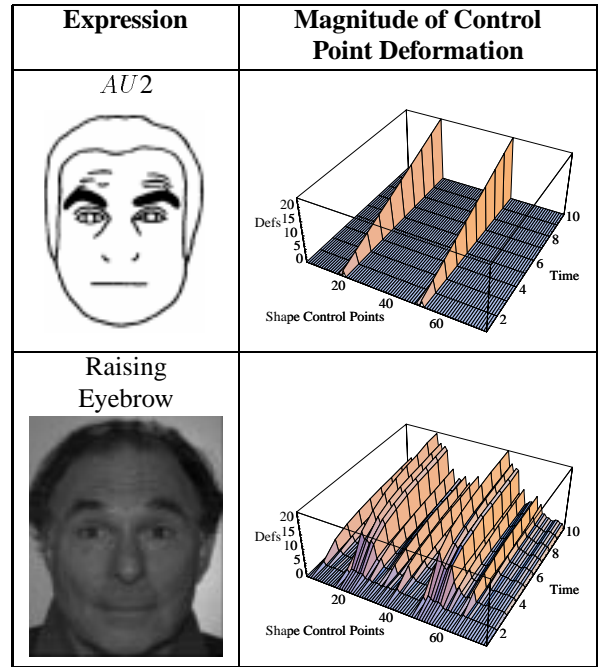
Figure 5. FACS/Candide deformation vs. Observed deformation for the Raising Eyebrow expression. Surface plots (top) show deformation over time for FACS actions AU2, and (bottom) for an actual video sequence of raising eyebrows.
