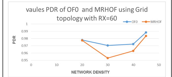
Fig. 36: PDR of OF0 and MRHOF using Grid topology.
