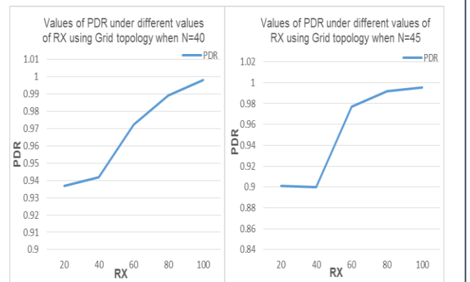
Fig. 9: PDR under different RX When N=40. Fig. 10: PDR under different RX When N=45.
