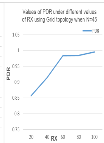
Fig. 26: PDR under different RX When N=45.
