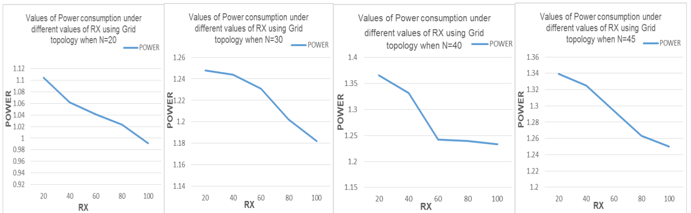
Fig. 15: Power under different RX When N=20. Fig. 16: Power under different RX When N=30. Fig. 17: Power under different RX When N=40 . Fig. 18: Power under different RX When N=45.
