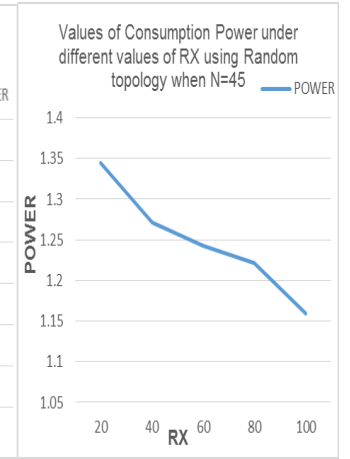
Fig. 30: Power under different RX when N=45.
