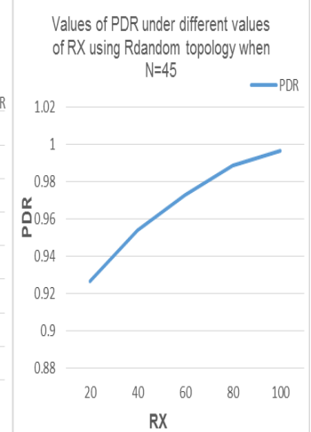
Fig. 22: PDR under different RX when N=45.
