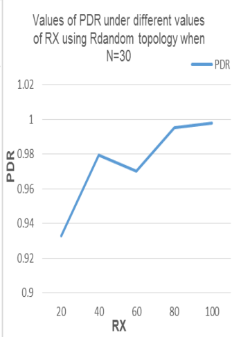
Fig. 20: PDR under different RX when N=30.
