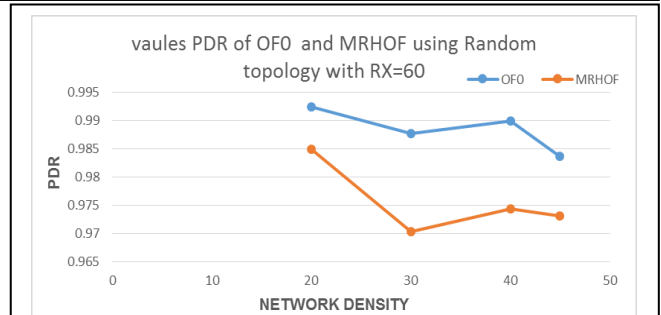
Fig. 35: PDR of OF0 and MRHOF using Random topology.
