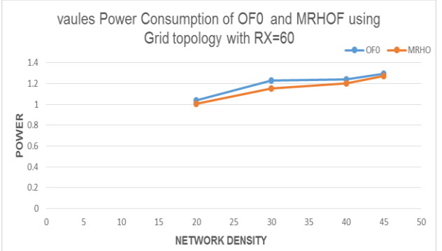
Fig 38: POWER of OF0 and MRHOF using Grid topology.
