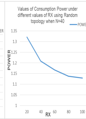
Fig. 29: Power under different RX when N=40 .
