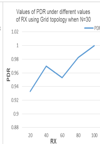
Fig. 24: PDR under different RX When N=30.
