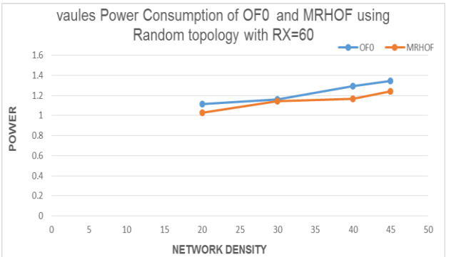
Fig 37: POWER of OF0 and MRHOF using Random topology.
