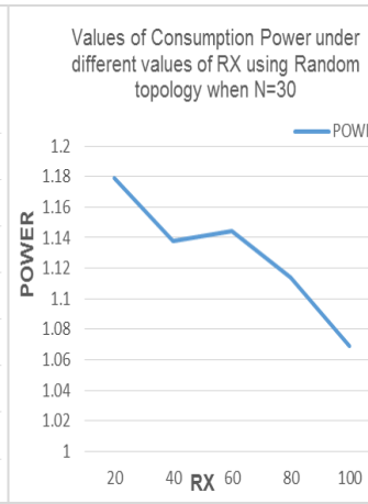
Fig. 28: Power under different RX when N=30.
