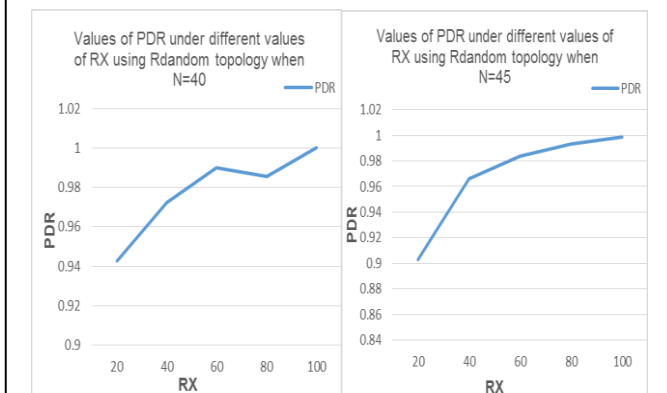
Fig. 5: PDR under different RX When N=40. Fig. 6: PDR under different RX When N=45.
