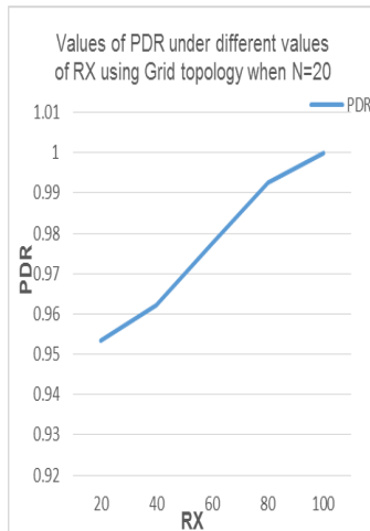
Fig. 23: PDR under different RX When N=20.
