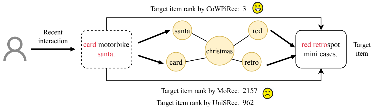
Fig. 3. The interaction history of a user in the “Online Retail” dataset, a sub-graph of our constructed word graph, and the rank results of the target item of models in the zero-shot setting. The word “card” and “santa” have co-click relationships with “retro” and “red” in the word graph. CoWPiRec utilizes the word-level CF signal learned from the word graph and captures “red” and “retro” in the target item. Therefore, CoWPiRec ranks the target item at a high position and achieves a clearly better performance than other models.
