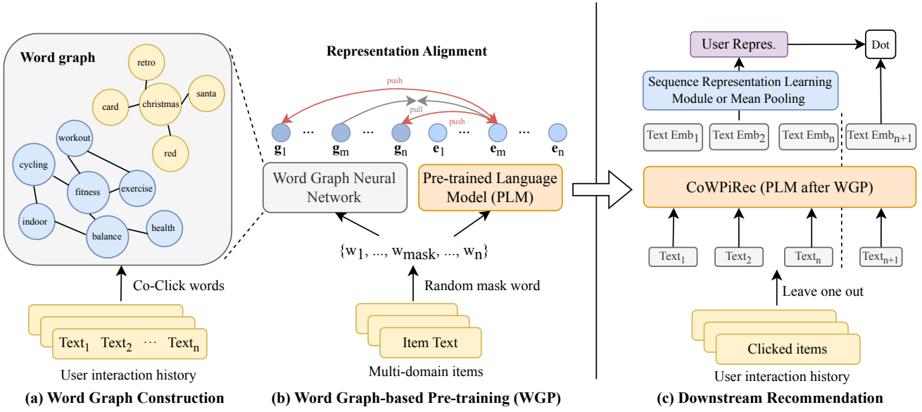
Fig. 1. The overall framework of our proposed collaborative word-based pre-trained item representation for recommendation (CoWPiRec). (a) The word-level collaborative filtering (CF) signals are from the co-click relationships of word pairs in the word graph. (b) A word graph-based pre-training (WGP) is performed to align the semantic- and the CF-related representation of the PLM and word graph with contrastive learning. w_i denotes the word in item text, g_i and e_i is the word representation after word graph modeling and semantic modeling (c) When transferring CoWPiRec to a new domain, the item representations generated offline utilizing CoWPiRec are fed into a sequence representation learning (SRL) module or a simple mean-pooling to perform downstream recommendations in the fine-tuning and zero-shot settings, respectively.
