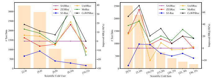
Fig. 2. Performance comparison in cold user and cold item experiment on “Scientific” dataset. The bar graph represents the number of users or items in test data for each group. The line chart represents the improvement ratios for HR@10 compared with SASRec.
