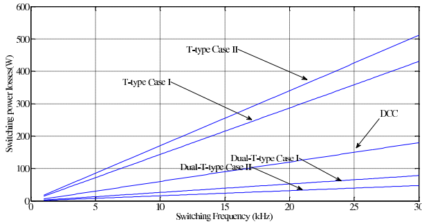
Figure 13: Switching losses for the dual-T-type converter compared to five-level DCC and T-type converter
