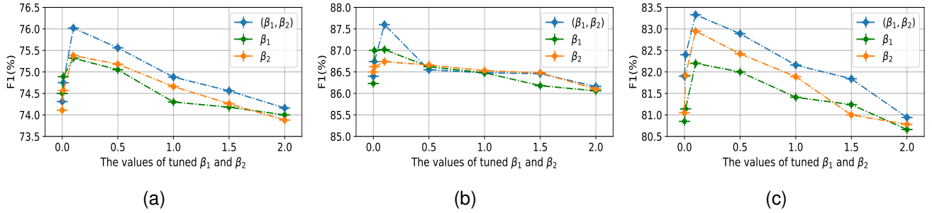
Fig. 4. The change F1 for our model with different values of \beta_1 and \beta_2 under different datasets: (a) The change of F1 on Twitter15 dataset; (b) The change of F1 on Twitter17; (c) The change of F1 on MRE dataset
