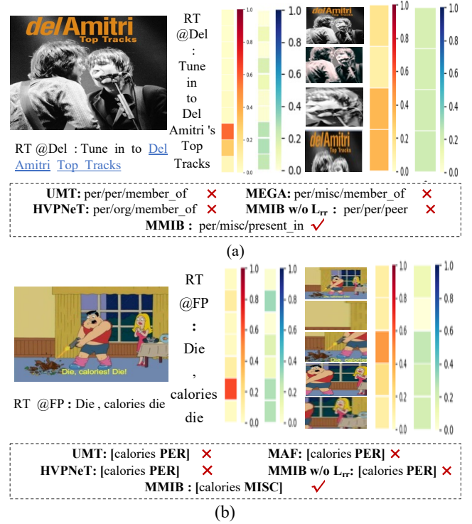
Fig. 3. Case study for modality-noise.
