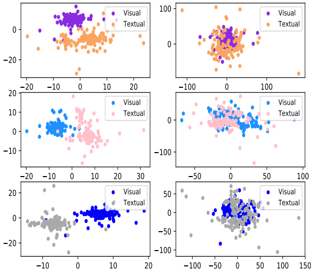
Fig. 5. Representation visualization to modality-gap.
