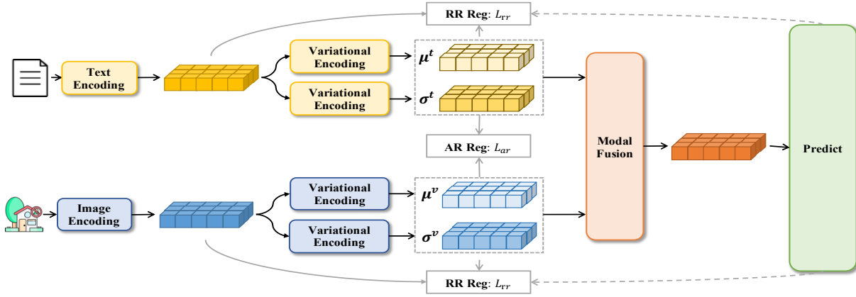
Fig. 2. Model Architecture.
