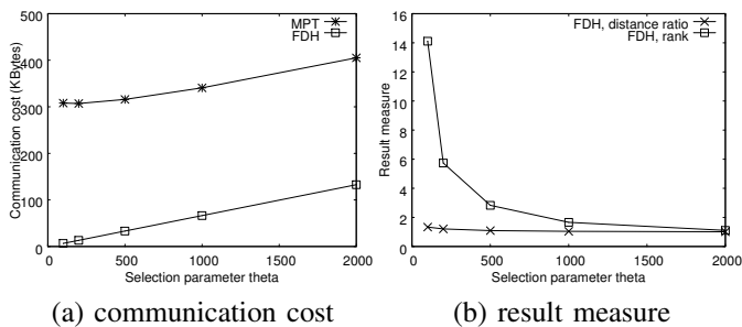
Fig. 10. Effect of \theta , on GFC data
