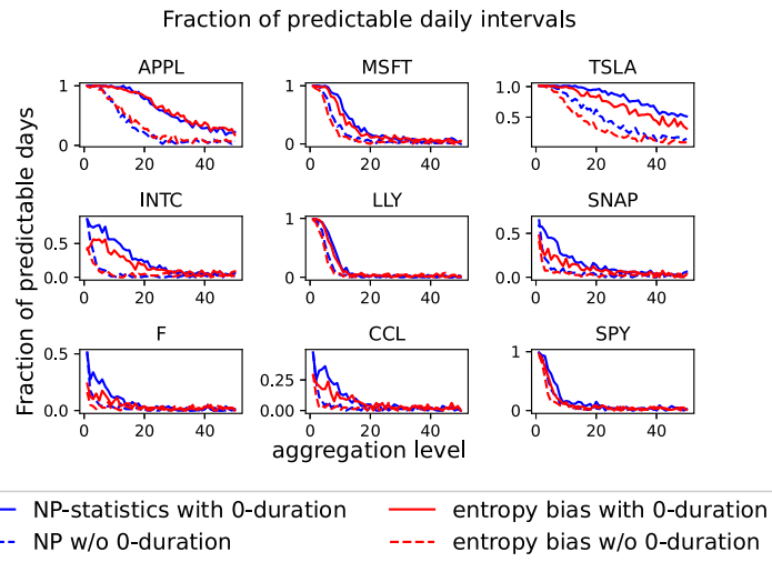
Fig. 7. Fraction of predictable days for different assets with and without simultaneous transactions.
