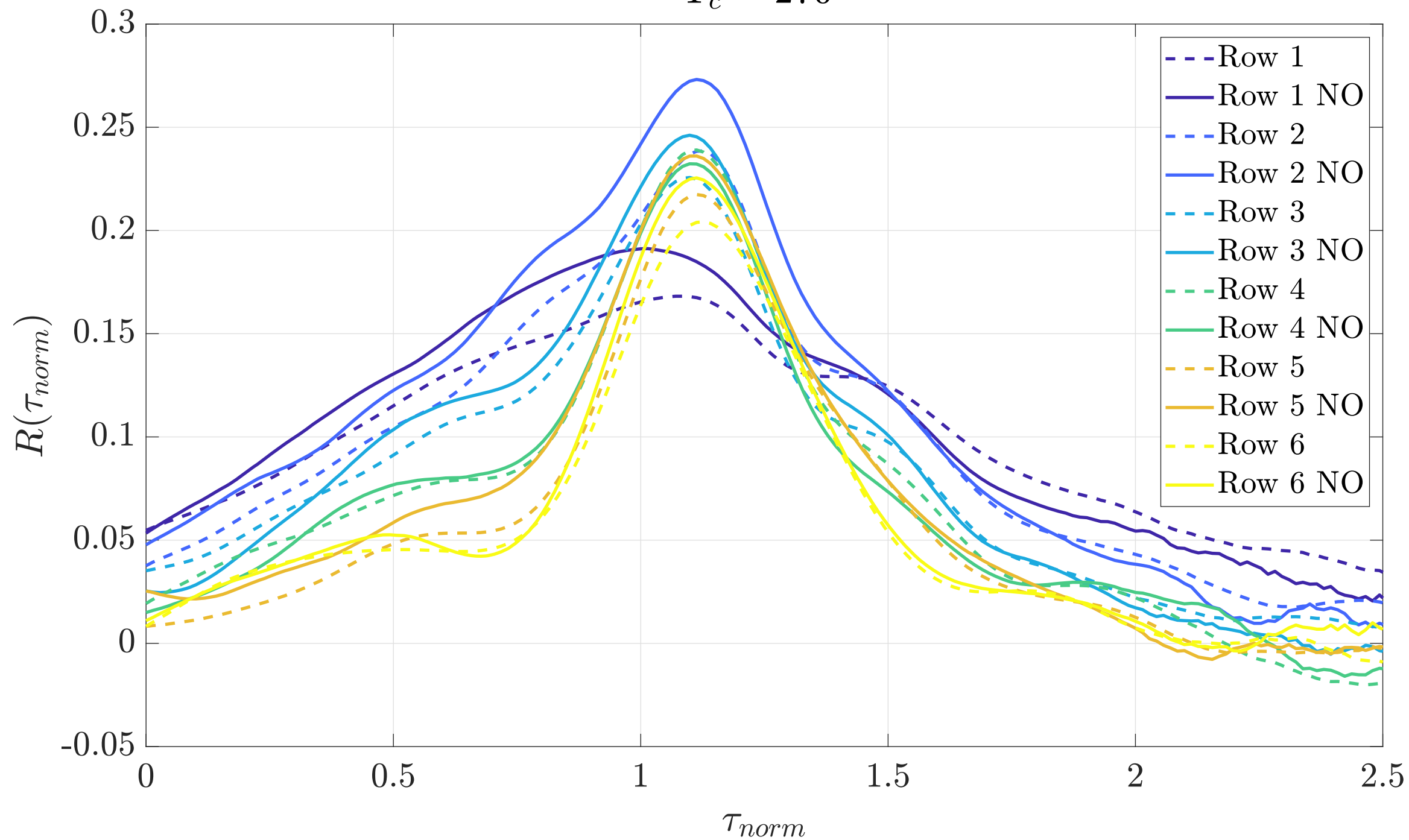
(a) Average power output fluctuation correlation per wind farm row.
