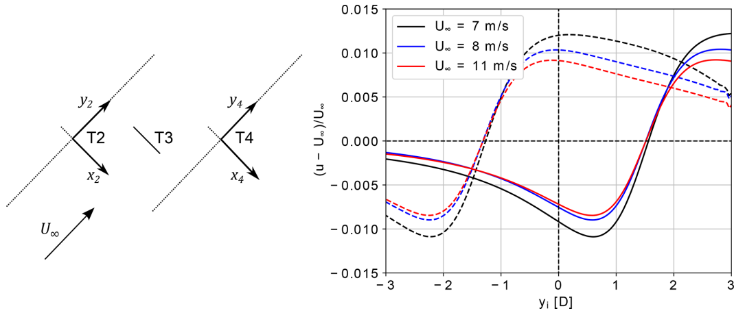
Figure 6. Velocities induced by the central turbine (T3) on the rotor axis of T2 (solid line) and T4 (dashed line), for different values of U_\infty , turbine inter-spacing of 2 D and \theta = 45^\circ .
