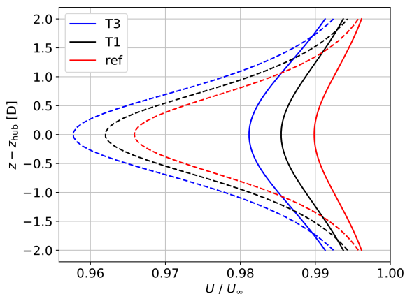
Figure 5. Upstream vertical velocity profiles extracted from RANS-CFD at 1D (dashed lines) and 2D (continuous lines) of the isolated case, T1 and T3 for U_\infty = 8 \text{ m s}^{-1} and \theta = 0^\circ .
