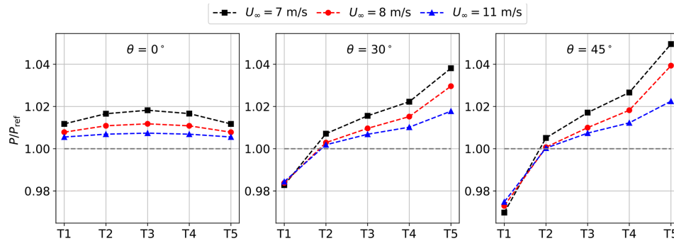
Figure 3. Power output of the five turbines normalised by that of an isolated turbine (placed at T3) for the cases with an inter-spacing of 2 D predicted by RANS–CFD.
