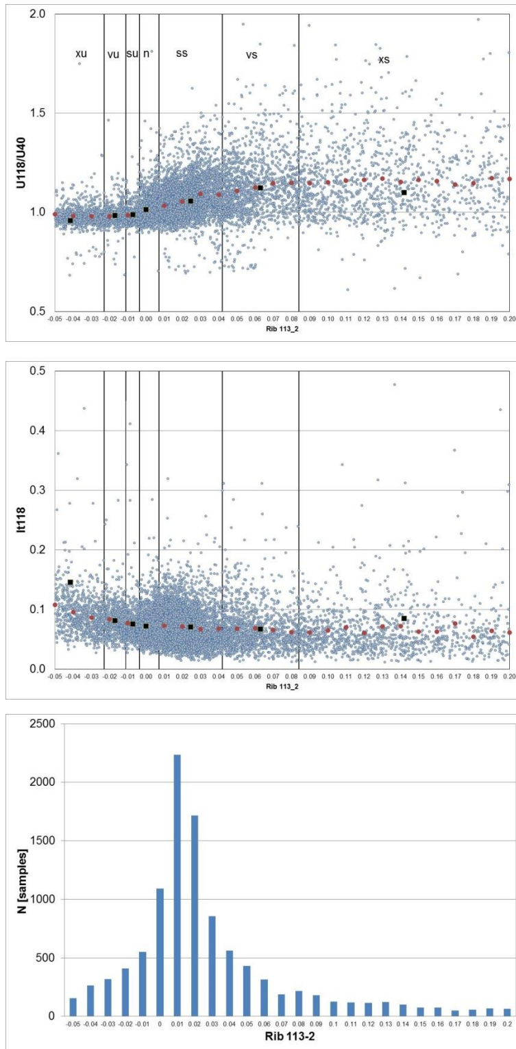
Figure 1 Wind shear and turbulence intensity vs Rib-based stability in MP5, [337.5°-22.5°] sector. Red dots are the Rib mean values for 0.01 resolution scale, black squares are the Rib mean values in each of the stability classes according to (Mohan, 1998).
