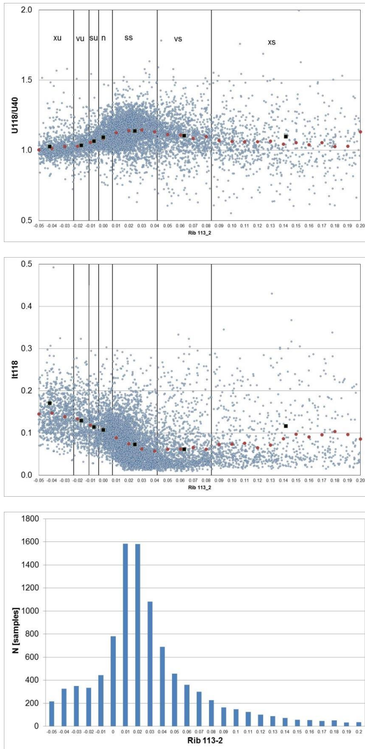
Figure 2 Wind shear and turbulence intensity vs Rib-based stability in MP5 , [157.5°-202.5°] sector. Red dots are the Rib mean values for 0.01 resolution scale, black squares are the Rib mean values in each of the stability classes according to (Mohan, 1998).
