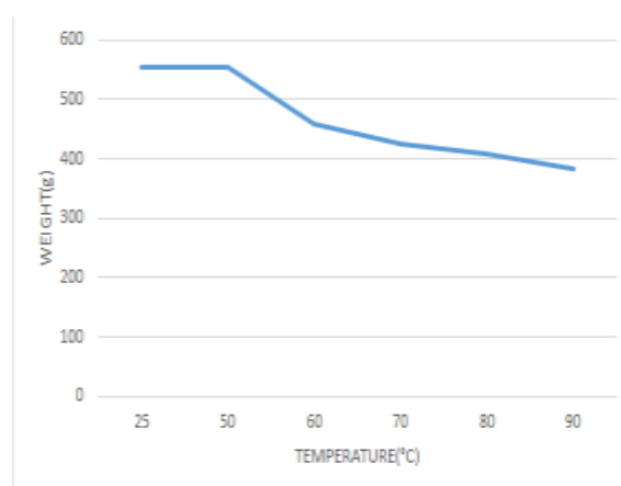
Fig. 4: Thermogravimetric analysis
