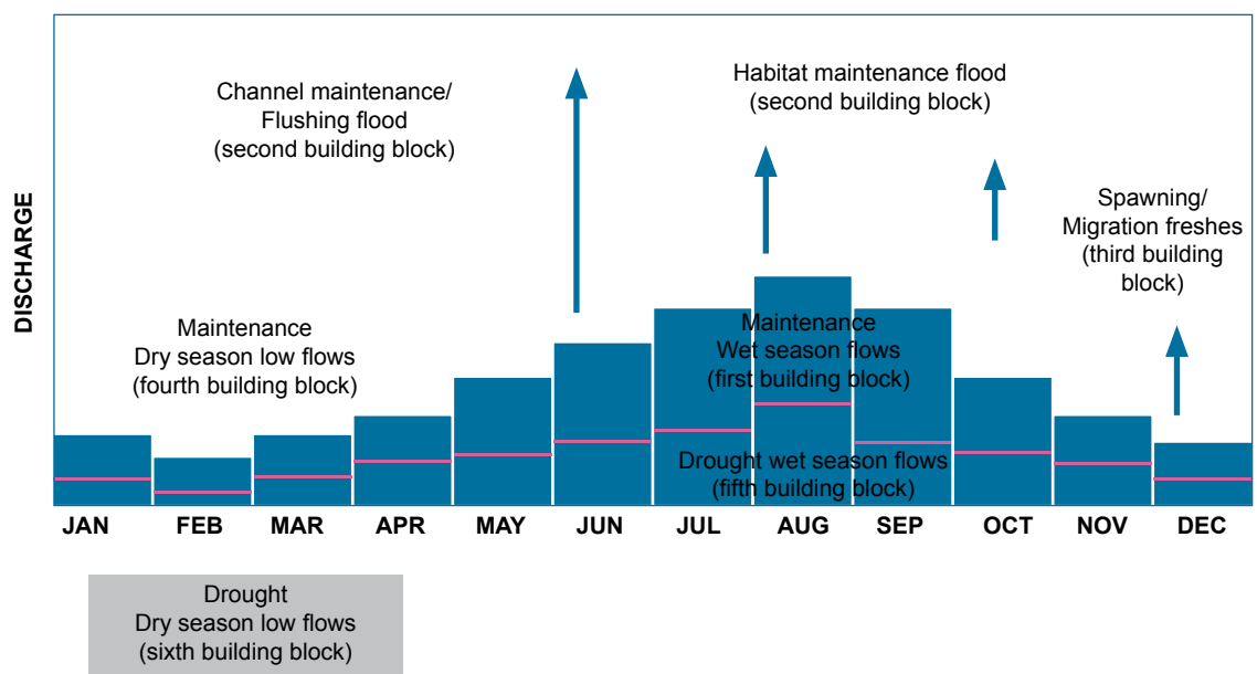
Figure 3: River Building Blocks classify the most critical elements of the flow regime needed to maintain physical and biological processes. Both habitat maintenance and channel maintenance floods compose the second building block.
