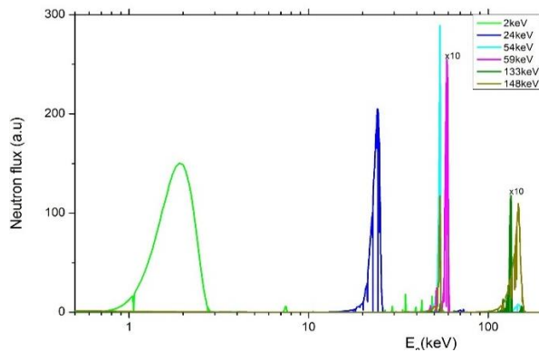
Fig. 2. The keV filtered neutron energies calculated by MCNP.
