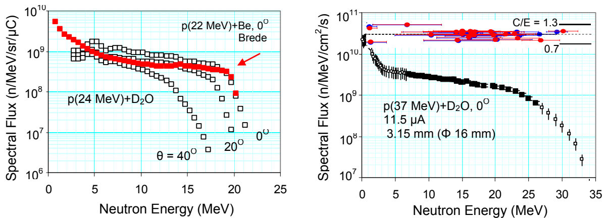
Fig. 2. Left: spectral neutron yield from p(24\text{ MeV})+D_2O reaction measured by scintillation detector; zero-degree spectral yield from p(22\text{ MeV})+Be reaction is given for a comparison. Right: p(37\text{ MeV})+D_2O spectrum obtained by activation technique and SAND-II adjustment procedure; in upper part - resulting C/E ratios for different dosimetry reactions displayed at energies weighted with product of neutron flux and corresponding cross-section.
