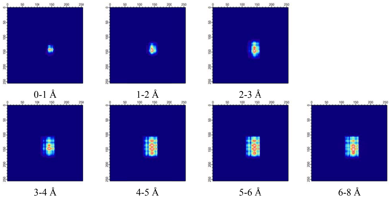
Fig. 3. Cuts from the 3D (X-Y-t) matrix for the shown Angstrom region corresponding time regions. The white square shows about a 2 cm x 2 cm area that is equal with the collimator sizes situated upstream of the beam, before the chopper blade. Repeated square regions in the figures belong to reflection of the neutron beam on the mirror walls. The guide is curved to the right looking in the directions of the neutrons. The picture shows the absorbed neutron positions from looking to it from the beam direction. The pinhole geometry reverses the up-down and left-right directions.
