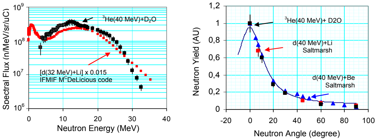
Fig. 1. Left: zero-degree spectral neutron yield from D_2O(^3He,xn) reaction compared to the Li(d,xn) spectrum calculated for IFMIF. Right: relative angular dependence of neutron yield from D_2O(^3He,xn) reaction versus experimental data for d+Li and d+Be reactions.
