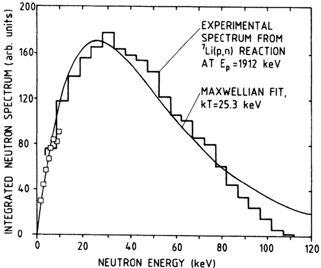
Fig. 1: The quasi-stellar neutron spectrum produced by the {}^7\text{Li}(p,n){}^7\text{Be} reaction at a proton energy E_p = 1912 \text{ keV} after integration over all emission angles (histogram and symbols) compared to a true thermal spectrum for kT = 25 \text{ keV} (from Ref. [1]).
