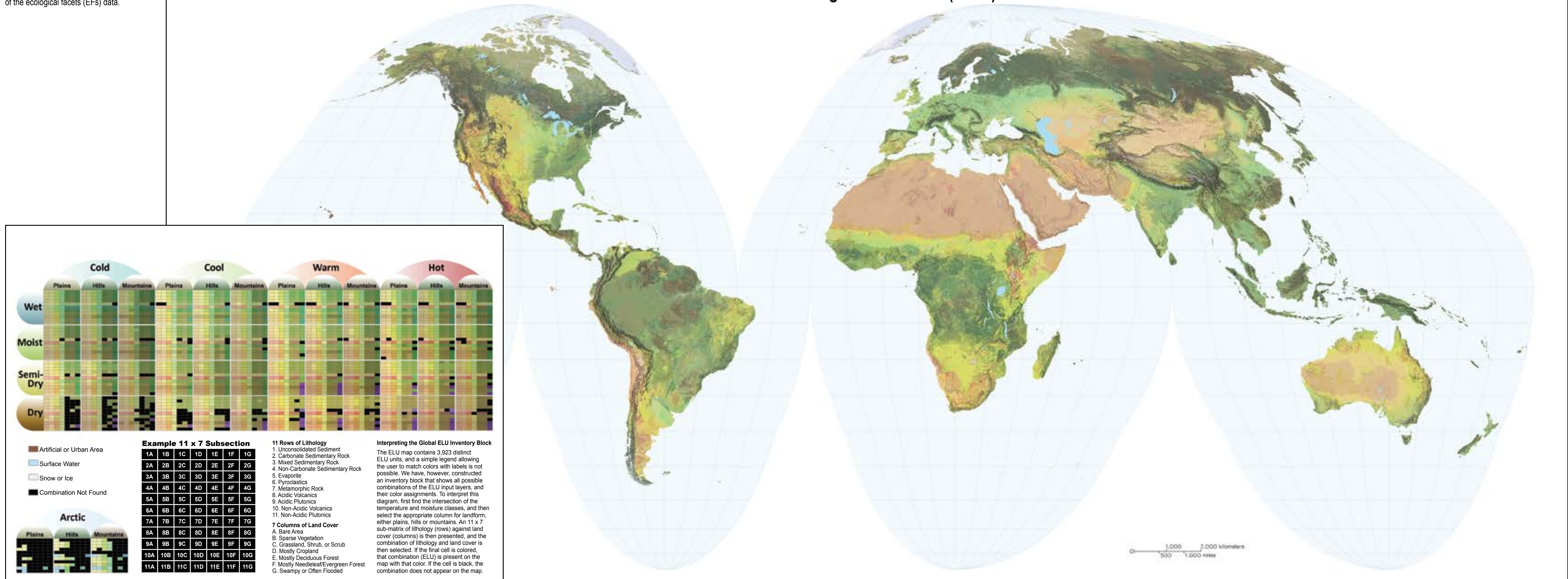
Figure 7. Map of global ecological land units (ELUs) produced as an aggregation of the ecological facets (EFs) data.
