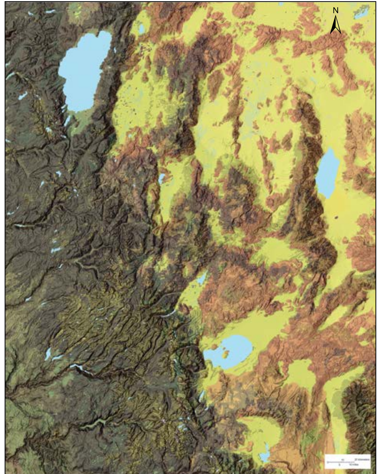
Figure 15. Map of ELUs of the Eastern Sierra Nevada Mountains region, southwestern United States.
