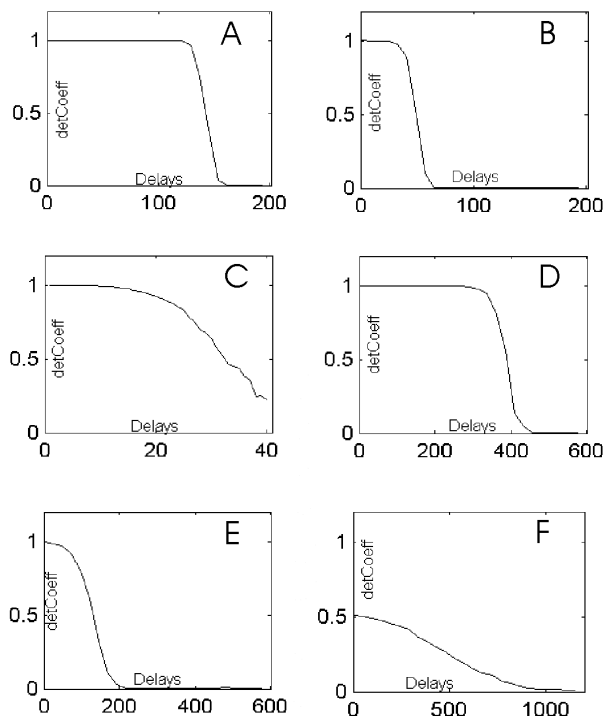
Figure 7.3: Forgetting curves of various 400-unit networks. A: randomly created linear DR. B: randomly created sigmoid DR. C: like A, but with noisy state update of DR. D: almost unitary weight matrix, linear update. E: same as D, but with noisy state update. F: same as D, but with spectral radius \alpha = 0.999 . Mind the different scalings of the x-axis!
