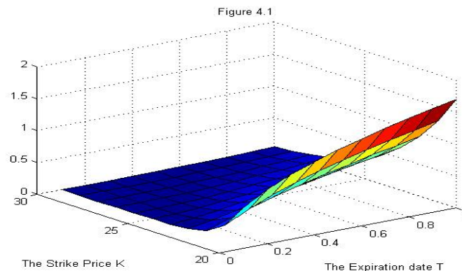
Figure 1. The price of a fixed strike geometric average Asian call option in subdiffusive regime V_\alpha(K, T) , according to the exercise date T and strike price K . Here, S_0 = 20, r = 0.06, \sigma = 0.3, \alpha = 0.8 .
