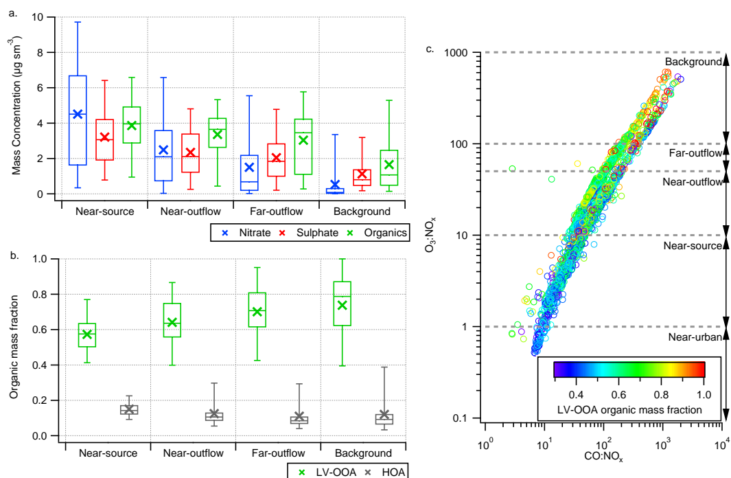
Fig. 7. Boxplot summary statistics of aerosol chemical composition as a function of proximity to source and photochemical processing. (a) Summarises the concentrations for nitrate, sulphate and organics, while (b) presents the organic mass fractions of LV-OOA and estimated HOA. Crosses represent the mean value, while horizontal lines represent the 25th, 50th and 75th percentiles. The whiskers represent the 5th and 95th percentiles. Values in (a) and (b) are for altitudes between 250–2500 m. (c) Summary of the relationship between the O_3:NO_x ratio and the CO:NO_x ratio for the dataset except for ADIENT-2 where no CO measurement was available. The grey horizontal lines designate the boundaries of the source proximities based upon the O_3:NO_x ratio which are used in (a) and (b). The points are coloured according to the LV-OOA organic mass fraction.
