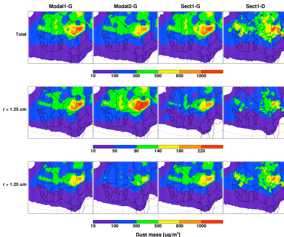
Fig. 6. Daytime (09:00–16:00 UTC) dust mass concentrations below 1 km a.g.l. for the simulation period over North Africa from the WRF-Chem simulations in four cases: Modal1-G, Modal2-G, Sect1-G, and Sect1-D. The mass concentrations are shown for dust particles in the whole size range ( r < 5 \mu\text{m} ), fine dust particles ( r < 1.25 \mu\text{m} ), and coarse dust particles ( 1.25 \mu\text{m} < r < 5 \mu\text{m} ), respectively.
