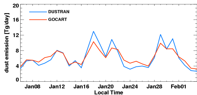
Fig. 4. Daily total dust emissions from the Dustran and Gocart schemes in Sect1-G and Sect1-D cases over North Africa for the simulation period.
