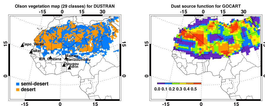
Fig. 1. Spatial distribution of desert and semi-desert masks determined by the Olson World Ecosystem database (29 classes) for the DUSTRAN scheme and the dust source function (Ginoux et al., 2001) for the GOCART scheme over North Africa. The black triangles represent the locations of the six AERONET sites. The Niamey airport, 60 km northwest from the Banizoumbou site, is also shown with the same triangle as Banizoumbou.
