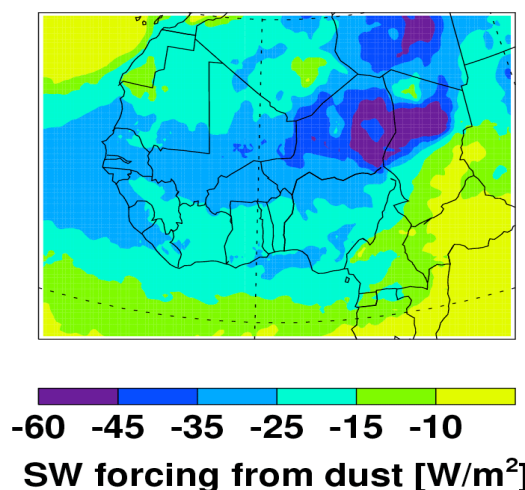
Fig. 12. Clear-sky surface SW dust radiative forcing at 12:00 UTC over North Africa for the simulation period estimated from the WRF-Chem simulations in the Sect1-G case. The SW dust radiative forcing is estimated by subtracting the result from the simulation without dust emissions from that from the simulation with dust emissions.
