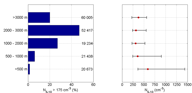
Figure 6. Statistics on the detection of significant particle concentration in the size range 5–10 nm as a function of altitude (left panel; the number of data points is indicated on the plot for each altitude range). Corresponding median concentrations are reported on the right panel; left and right limits of the error bars stand for the 1st and 3rd quartile, respectively.
