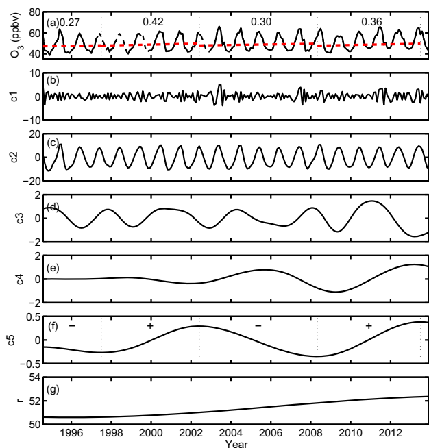
Figure 6. The interpolated monthly average ozone mixing ratio at WLG from 1994 to 2013 (the interpolated data given in dashed lines, a ) and its intrinsic mode functions c_1 – c_5 ( b – f , from the lowest to the highest-order IMF) and its residue, r ( g ). The time segments in ( a ) were determined by the slope of the c_5 . The red slashed lines are the Theil–Sen trends and the numbers are the Theil–Sen trend estimates (in ppbv year -1 ).
