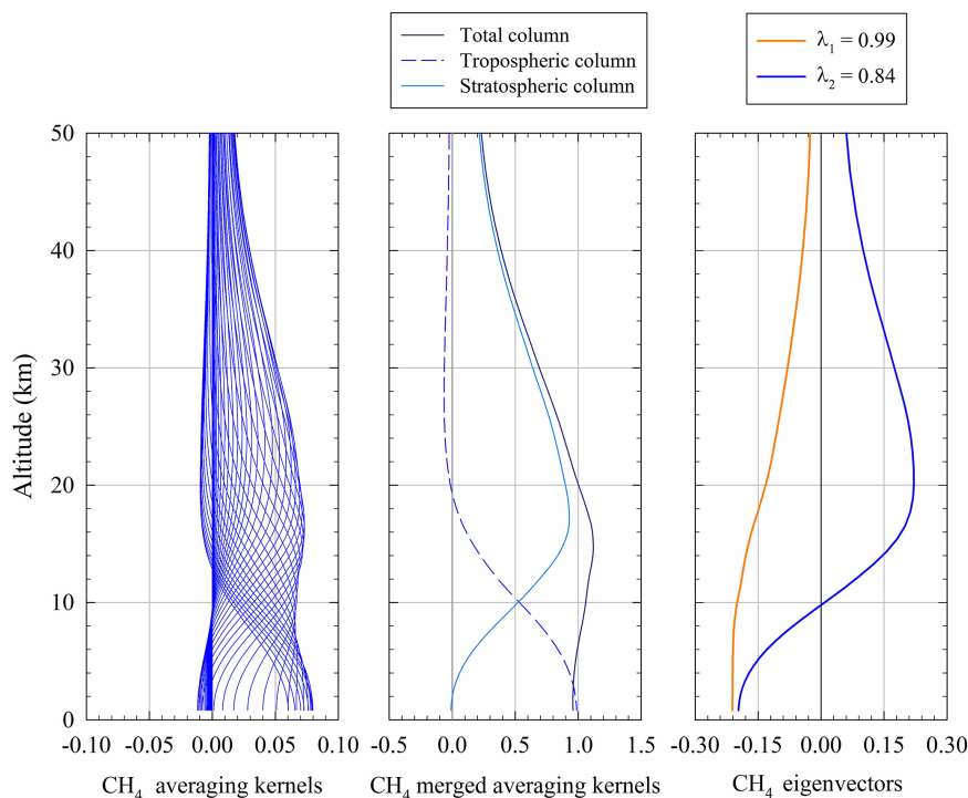
Figure 3. Typical NDACC methane retrieval. From left to right. First panel: typical individual (blue curves) \text{CH}_4 mixing ratio averaging kernels. Second panel: merged (shades of blue curves) \text{CH}_4 mixing ratio averaging kernels. For merged-layer kernels, corresponding atmospheric column are specified in the legend box. Third panel: corresponding two first eigenvectors. Associated eigenvalues are given in the legend.
