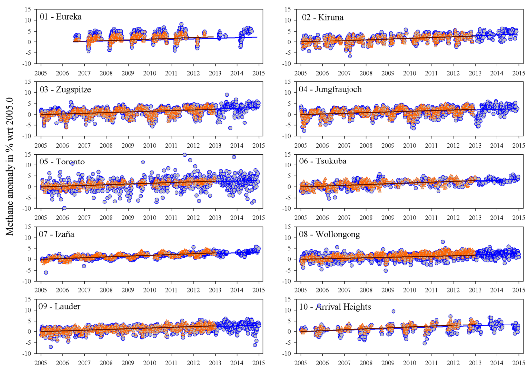
Figure 5. Daily mean CH 4 total column anomalies with respect to 2005.0 (in %) for 10 NDACC stations between 2005 and 2014 for NDACC FTIR observations (in blue) and between 2005 and 2012 for the smoothed GEOS-Chem simulation (in orange) along with their respective linear component of the bootstrap fit in blue and brown.
