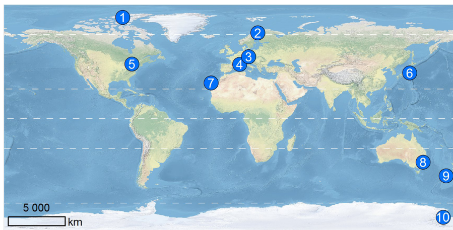
Figure 1. Map of all participating NDACC stations. Detailed coordinates of each station are provided in Table 1.
