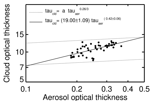
Figure 8. Cloud optical thickness as a function of aerosol optical thickness. The broken lines are the suggested dependencies of the two optical thicknesses assuming that ACI-I is valid. The solid line is the actual fit through the data.
