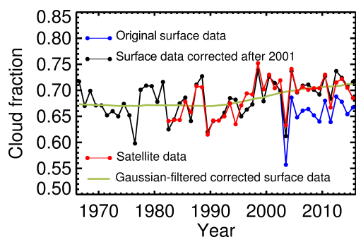
Figure 1. Surface-based cloud fraction estimates versus satellite-based estimates.
