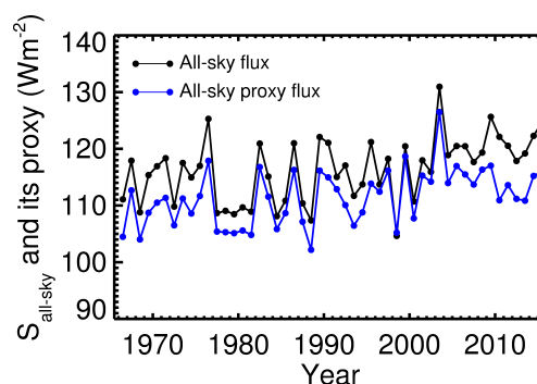
Figure 4. The all-sky radiation and its proxy.
