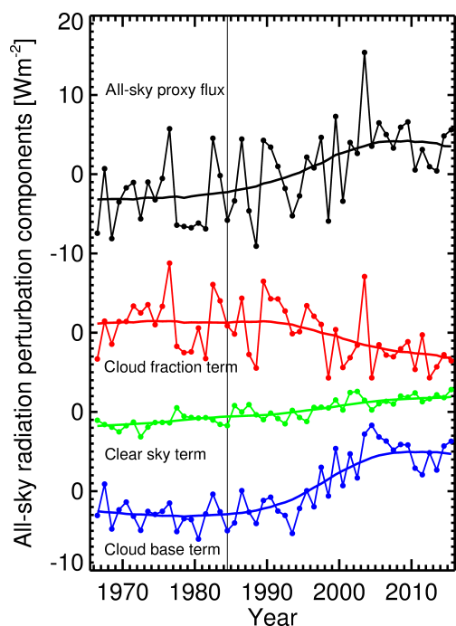
Figure 5. All-sky radiation perturbation components. Terms are indicated in the graph; 21-point Gaussian filter smoothers are drawn through the curves.
