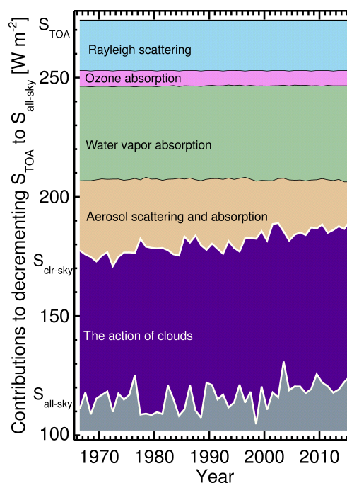
Figure 2. Impact on all-sky flux due to Rayleigh scattering, ozone absorption, water vapour absorption, aerosol scattering and absorption and the action of clouds.
