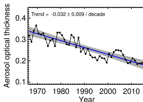
Figure 6. Aerosol optical thickness derived from visibility observations.
