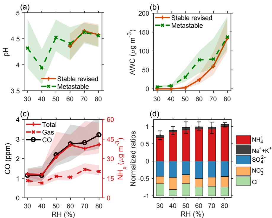
Figure 6. Variations of several chemical and physical parameters as a function of RH. (a–b) \text{PM}_{2.5} pH and AWC predicted from forward-mode ISORROPIA calculations in both stable and metastable states. (c) Measured concentrations of CO, total (gas plus aerosol) \text{NH}_x , and gas-phase \text{NH}_3 . For \text{NH}_3 , 1 \mu\text{g m}^{-3} \approx 1.3 \text{ ppb} at standard temperature and pressure. (d) Equivalent ratios of different ions normalized by the levels of total anions. The data are grouped in RH bins (10% increment). The shaded regions in (a)–(c) and error bars in (d) indicate the 25th and 75th percentiles. The measurement uncertainties of ions and gases are considered in pH and AWC calculations using a Monte Carlo approach.
