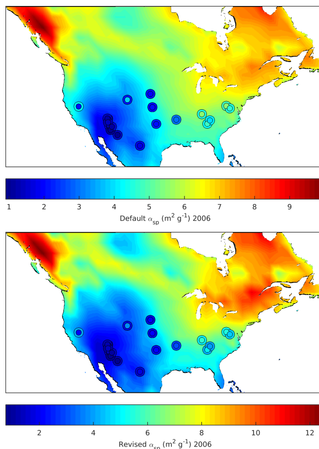
Figure 11. GEOS-Chem annual average mass scattering efficiency (at 550 nm) for the year 2006 using default and revised sizes and hygroscopicity for secondary inorganic and organic aerosols. Overlying inner circles represent annual averages of \alpha_{\text{sp}} at IMPROVE network sites for the year 2006. Outer rings represent coincident average simulated \alpha_{\text{sp}} .
