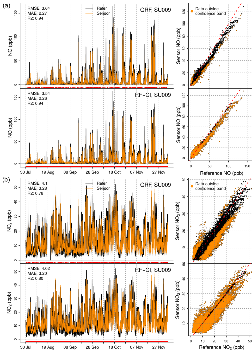
Figure 11. Comparison of QRF and RF-CI estimates of NO (a) and NO 2 (b) by SU009 with observations by reference instruments, at the urban background site Zurich-Kaserne. The grey shaded area indicates either the 5–95 % quantiles band (QRF case) or the 95 % confidence interval (RF-CI case). 1 : 1 red dashed line is added in the scatterplots.
