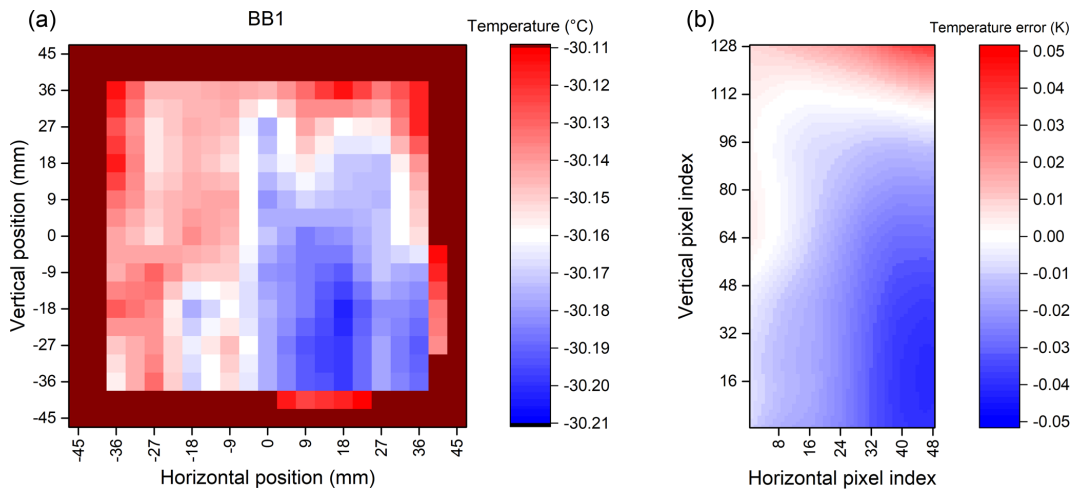
Figure 8. Measured surface radiance temperatures at -30.15\text{ }^{\circ}\text{C} (243 K) for BB1 (a) and estimated resulting temperature error for each of the 48 \times 128 detector pixels (b).
