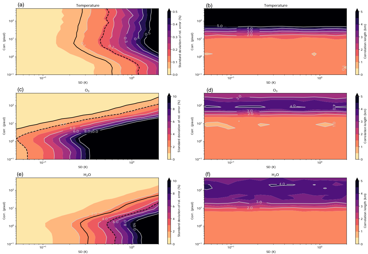
Figure 5. Results of the Monte Carlo approach. Plotted are the standard deviations (a) and correlation lengths (b) of the retrieval error distributions. The x axis shows the standard deviation of the original random variation of the blackbody temperature and the y axis shows the according correlation length. The top row represents the temperature retrieval, in the middle ozone is shown, and the bottom depicts water vapor. The black solid (dashed) line in the left plots indicates the error target (threshold) due to the long-term trend of the respective atmospheric species.
