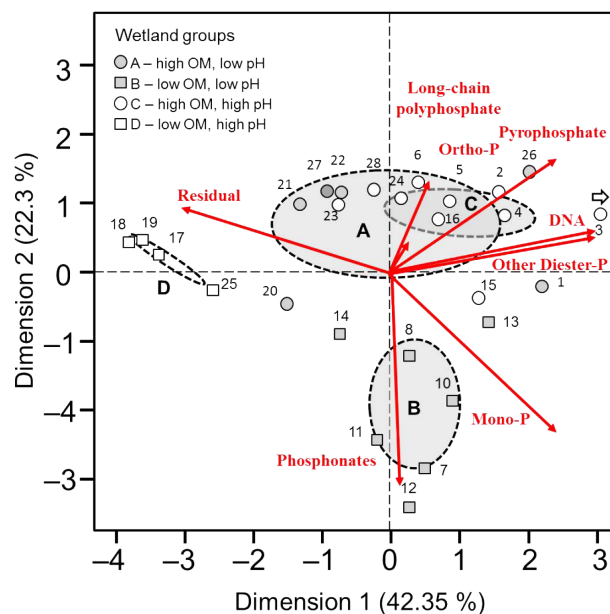
Figure 4. Biplot of the scaled first two principal components of phosphorus composition in wetland soils. Ellipses represent 95% confidence interval surrounding barycenter of four wetland groupings based upon pH and organic matter content. Proportional loading of P composition superimposed in red.
