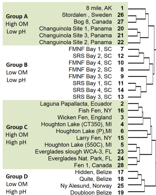
Figure 1. Wards hierarchical classification of 28 palustrine wetlands used to delineate four types of wetland (A–D) based upon organic matter (OM) content and pH. Francis Marion National Forest (FMNF), Savannah River Site (SRS).
