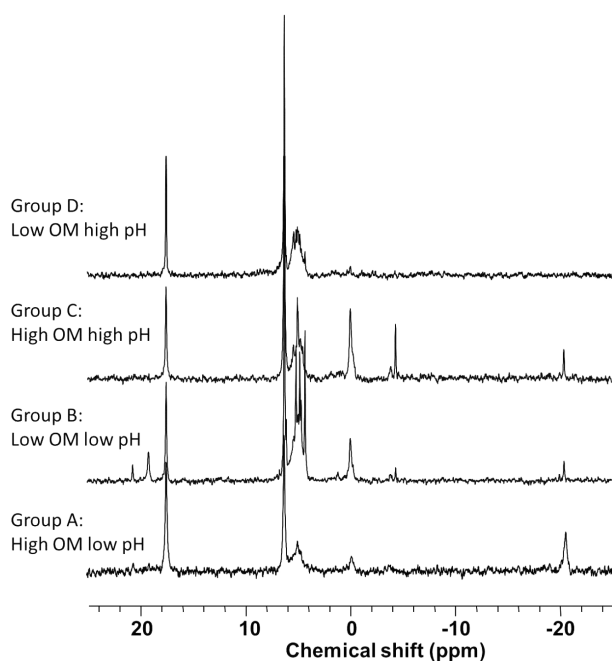
Figure 3. Solution ^{31}\text{P} NMR spectra of wetland soils representative of four wetland types identified in this study; see Figs. S1–S4 in the Supplement. Spectra acquired using an Avance III 500, Magnex 11.8 tesla 54 mm Bore, at \text{pH} > 13 , using a simple zgpg pulse program and calibrated 30^\circ pulse angle. Spectra presented here, using 15 Hz line broadening, scaled and referenced to internal standard methylenediphosphonic acid ( \delta = 17.46 ppm).
