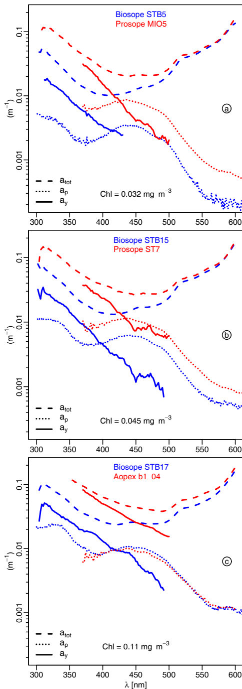
Fig. 8. Spectra of the total absorption coefficient ( a_{tot} ), derived from the diffuse attenuation coefficient, of the particulate absorption ( a_p ) determined via the glass fiber filter technique, and of the dissolved colored matter ( a_y , see text). (a) For a couple of stations in Pacific and Mediterranean waters (blue and red curves, respectively) with the same chlorophyll concentration, as indicated. (b) and (c) As in (a), but for other [chl] values. Note that during the Mediterranean cruises and because of technical limitations, the a_p determinations were restricted in the UV domain to 370 nm. Consequently, the a_y estimates experience the same spectral limitations. This limitation was removed for the BIOSOPE cruise.
