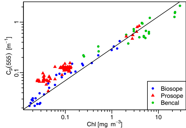
Fig. 5. The particle attenuation coefficient, c_p (as \text{m}^{-1} ) at the wavelength 555nm, obtained using an ac-9 instrument, and plotted as a function of [\text{Chl}] for the upper layer waters in the Pacific Ocean (blue dots) and in the Mediterranean Sea (red dots). The line represents the relationship c_p(555) = 0.275 [\text{Chl}]^{0.635} , derived from c_p(660) in Loisel and Morel (1998; their subsets 2 and 3), and by using a \lambda^{-0.5} dependency for the transfer from 660 to 555 nm.
