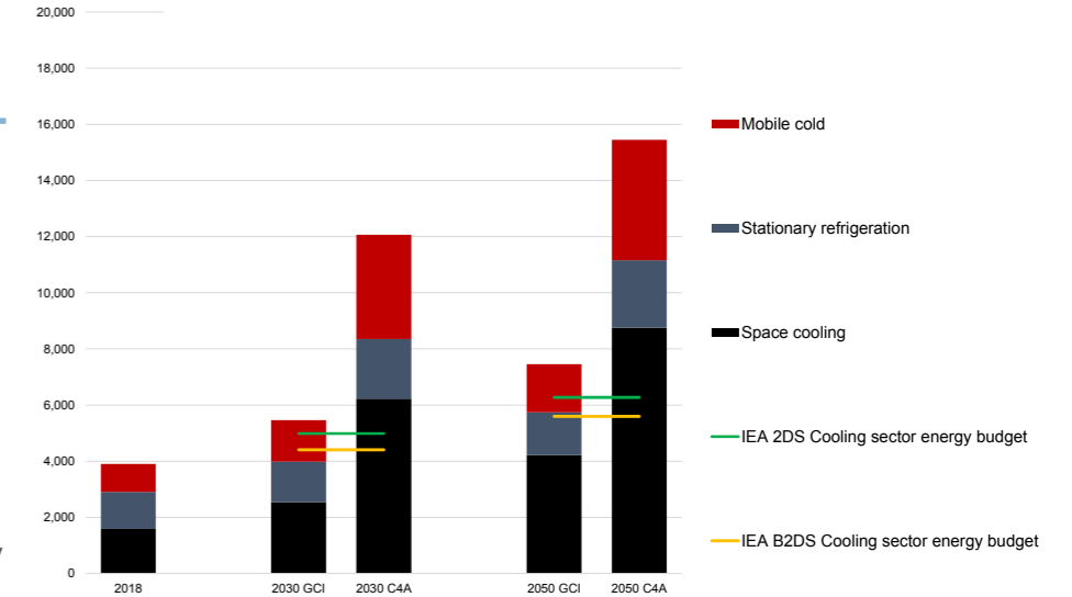
Total cooling sector energy consumption by sector in accelerated tech progress scenario (TWh/year)
