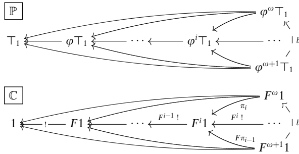
Fig. 1. Final sequences in a fibration.
