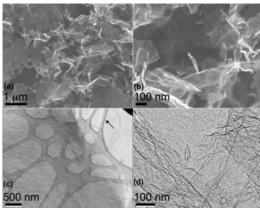
FIG. 4. SEM of the GA at low (a) and high (b) magnifications. TEM of the GA at low (c) and high (d) magnifications. Black arrow denotes hole carbon on TEM grid. Reproduced by permission from Ref. 9 (American Chemical Society).
