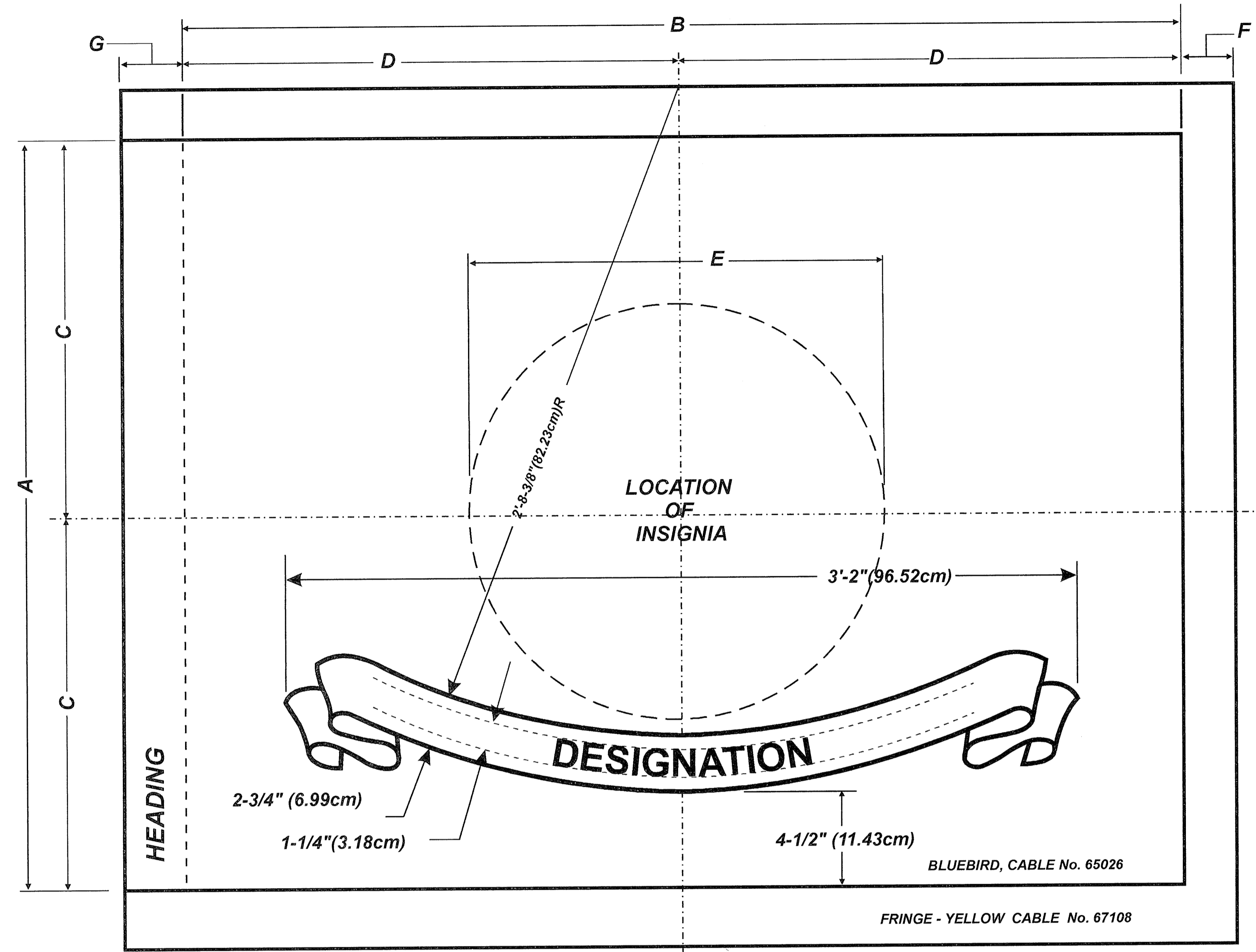
DRAWING IS SCALED FOR A 3' X 4' FLAG AT 3 INCHES = 1 FOOT
