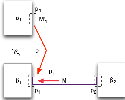
Fig. 3. The context of Theorem 29.
