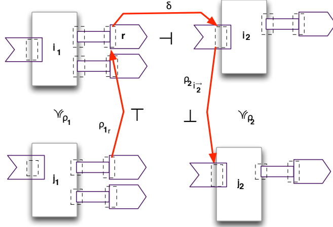
Fig. 12. The context of Theorem 52.
