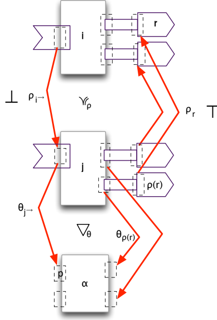
Fig. 11. The context of Theorem 51.
