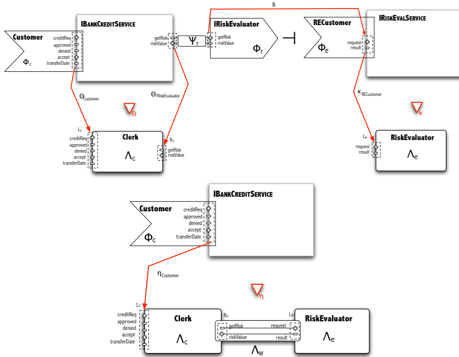
Fig. 10. The composition of two orchestrations.
