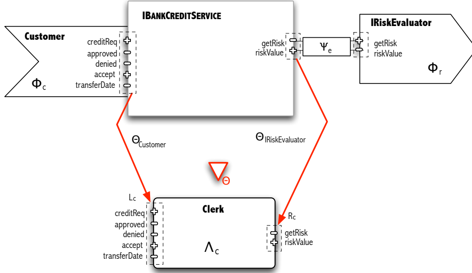
Fig. 6. Example of an orchestration: \nu_{Clerk} \triangleleft_{\Theta} IBANKCREDITSERVICE .
