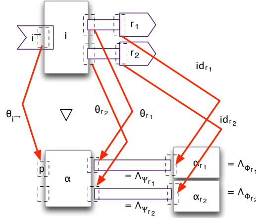
Fig. 5. \alpha \triangleleft_{\theta} i iff the properties in \Phi_{i \rightarrow} are validated by the composition of \alpha with the models of the specifications of the requires-points.
