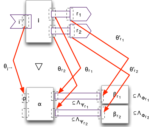
Fig. 7. \alpha \triangleleft_{\theta} i iff the properties offered through \Phi_{i \rightarrow} are validated by all compositions of \alpha with ARNs and via channels that validate the specifications of the requires-points.
