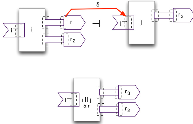
Fig. 8. Match between interfaces i and j and the interface that results from their composition.
