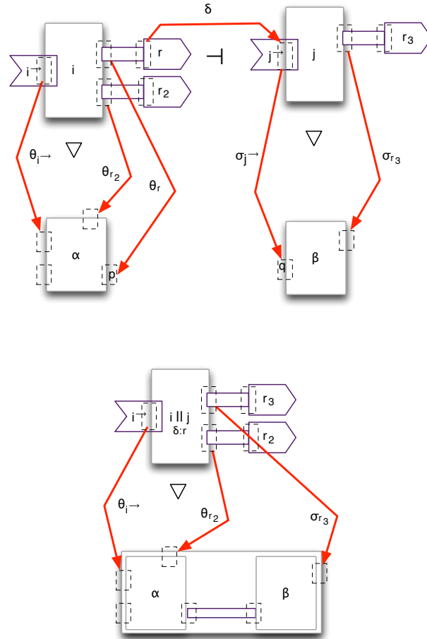
Fig. 9. The context of Theorem 48.
