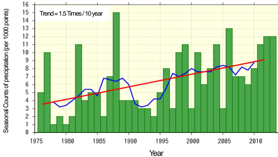
Figure A3 Seasonal number of events in summer (June – August) with precipitation exceeding 80 mm/hour from 1976 to 2013 (per 1,000 Automated Meteorological Data Acquisition System (AMeDAS) points)
